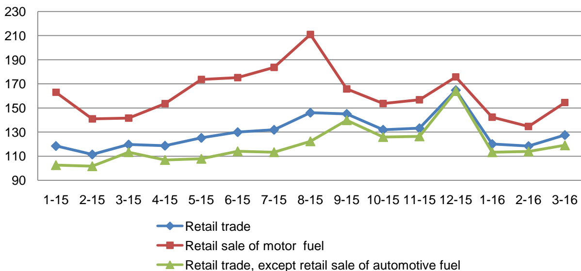
Fig. 1 Volume indices on Retail Trade and Retail Sale of motor fuel
